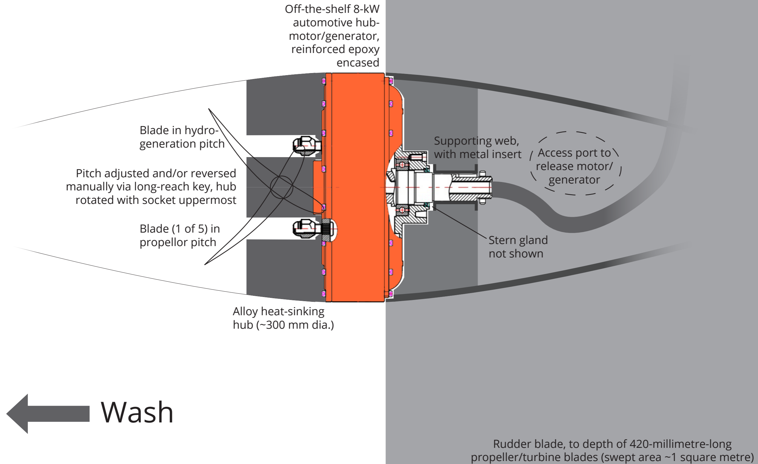
Marinised 8-kW electric automotive hub-motor/generator concept for Pūhoi river-mouth ferry
